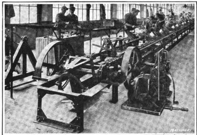
Fig. 28—Formerly the Packard Motor Car Co. assembled clutch units on stands that were distributed over the floor of the clutch assembling department. The Palmer-Bee Co. suggested that the progressive method of assembly be employed in handling them, so a conveyor system was installed, which carries stands similar to those formerly employed
